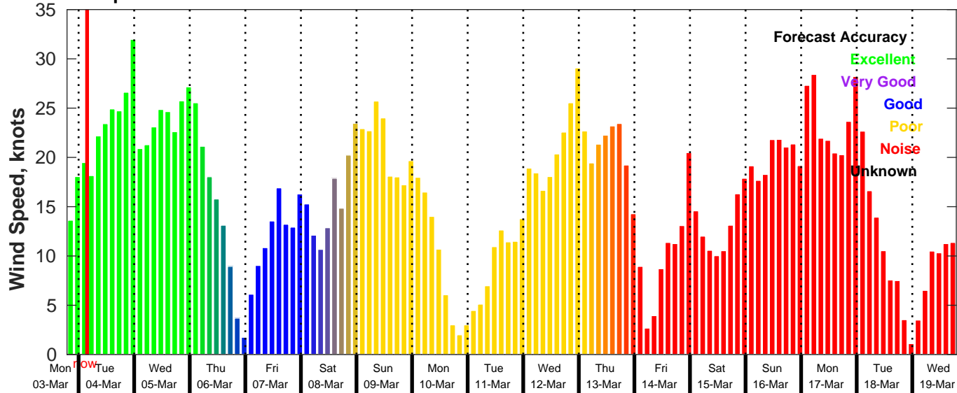
GFS Wind Speed Forecast for NDBC 42040 from 03-Mar-2025 19:00:00 to 19-Mar-2025 19:00:00
