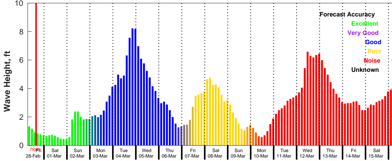
GFS Wave Forecast for NDBC 42084 from 28-Feb-2025 07:00:00 to 16-Mar-2025 07:00:00
