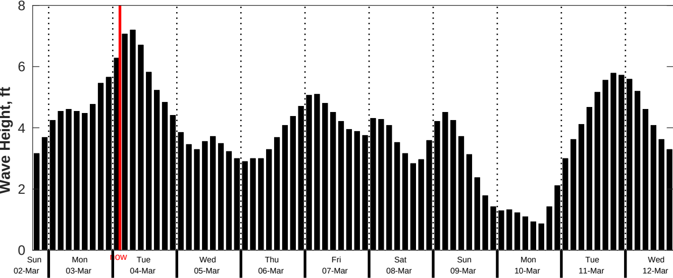
CMEMS Wave Forecast for NDBC 42092 from 02-Mar-2025 18:00:00 to 12-Mar-2025 18:00:00
