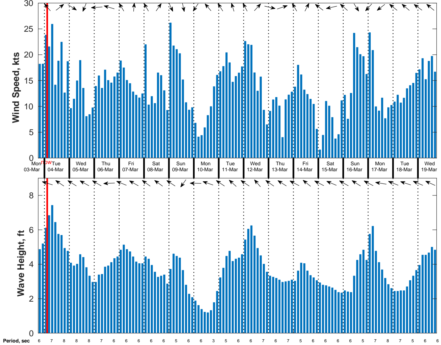
Wind & Wave Forecast for NDBC 42092 from 03-Mar-2025 18:00:00 to 19-Mar-2025 18:00:00
