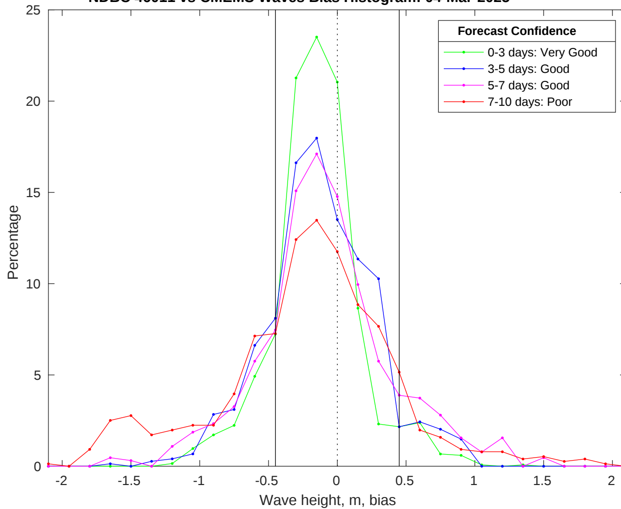
NDBC 46011 vs CMEMS Waves Bias Histogram: 04-Mar-2025
