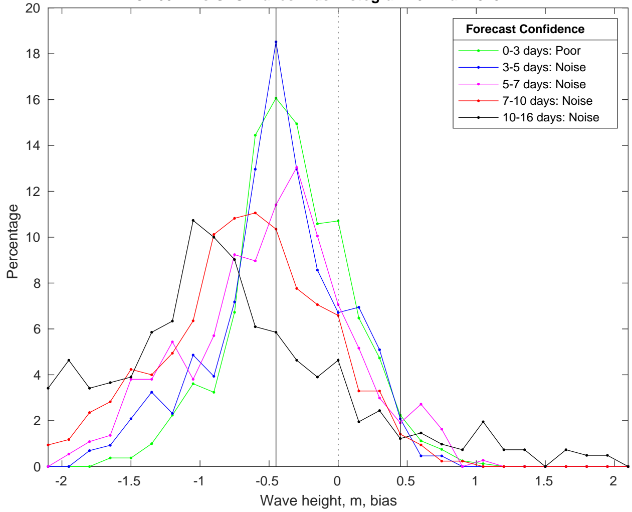
NDBC 46011 vs GFS Waves Bias Histogram: 04-Mar-2025
