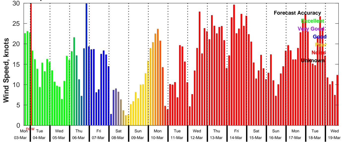
GFS Wind Speed Forecast for NDBC 46011 from 03-Mar-2025 16:00:00 to 19-Mar-2025 16:00:00
