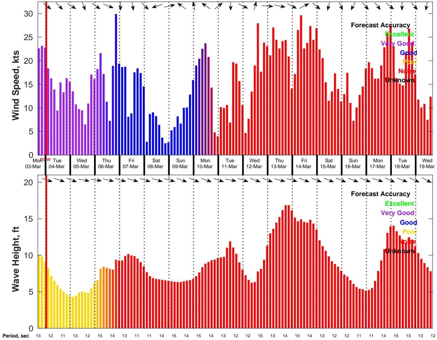
Wind & Wave Forecast for NDBC 46011 from 03-Mar-2025 16:00:00 to 19-Mar-2025 16:00:00
