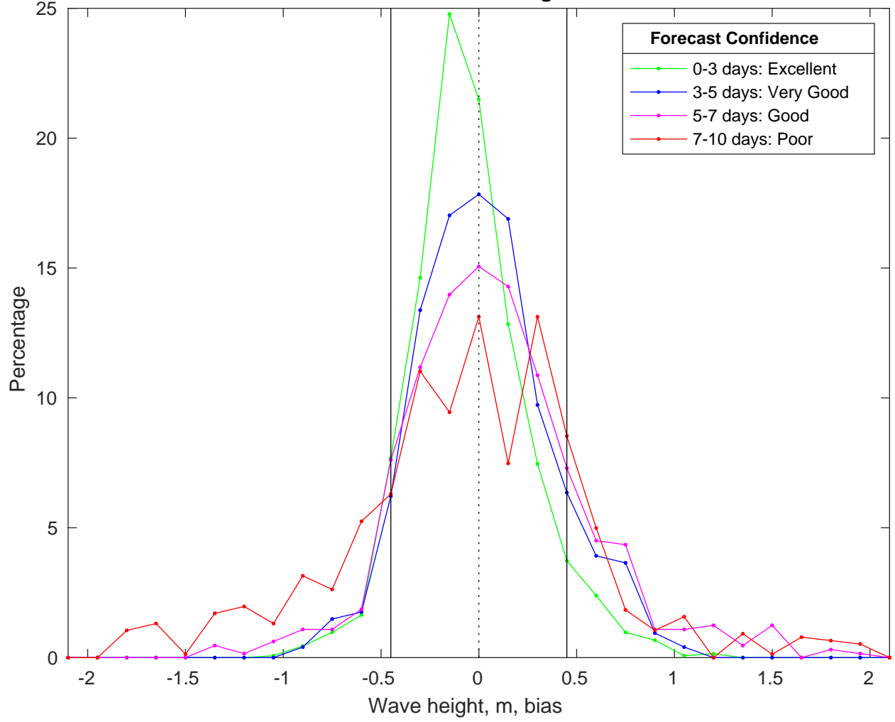
NDBC 46028 vs CMEMS Waves Bias Histogram: 04-Mar-2025
