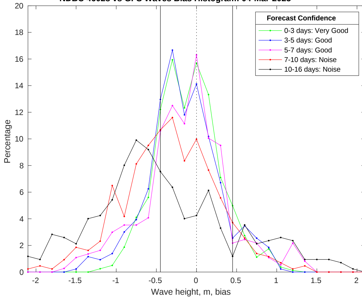
NDBC 46028 vs GFS Waves Bias Histogram: 04-Mar-2025
