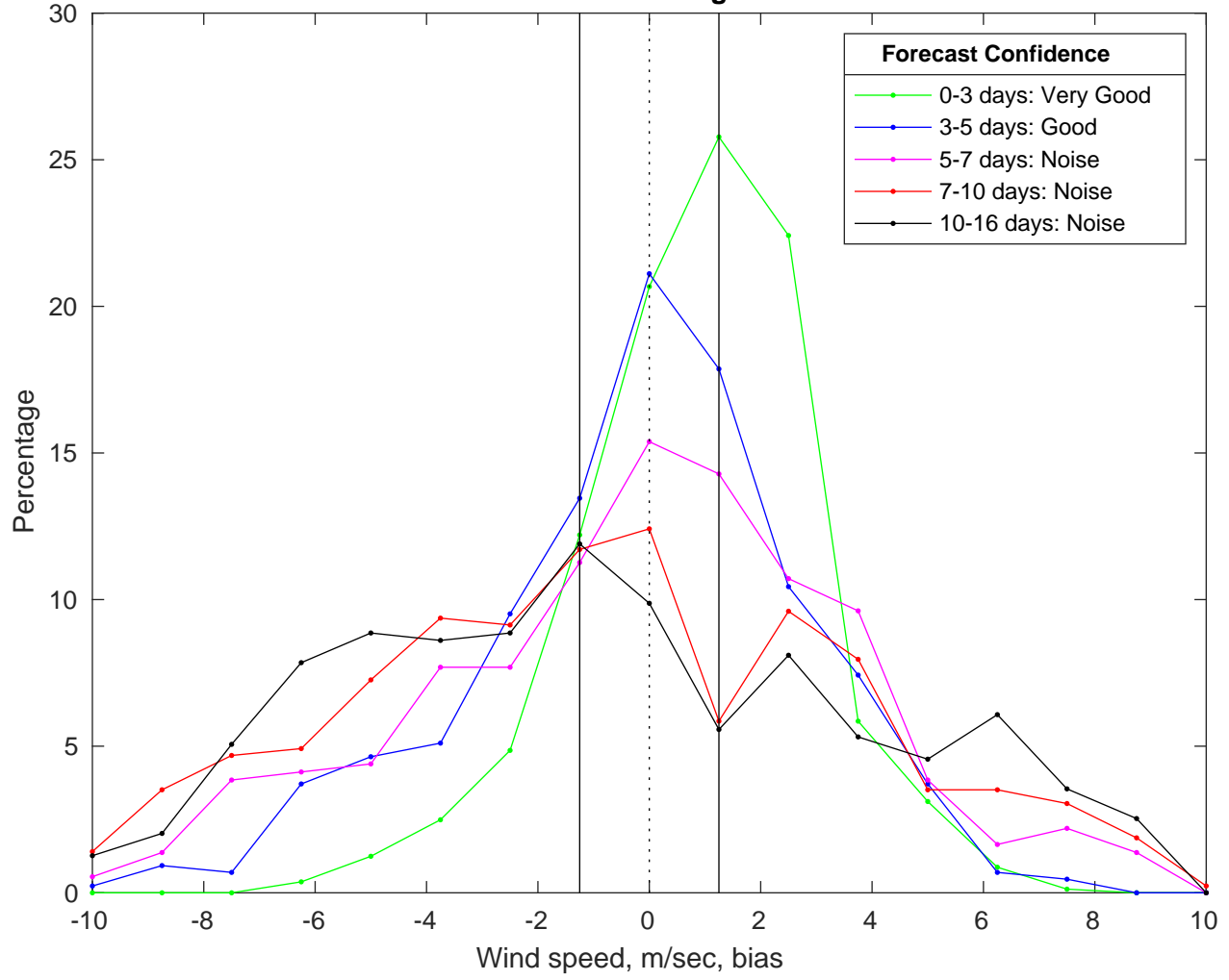
NDBC 46028 vs GFS Winds Bias Histogram: 04-Mar-2025
