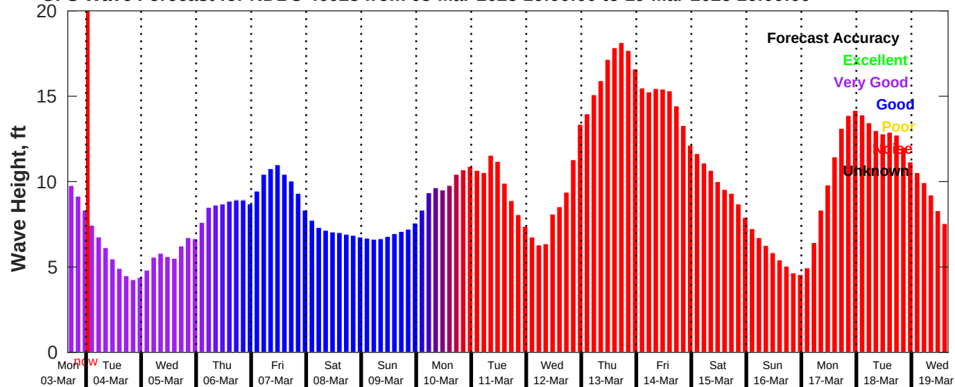
GFS Wave Forecast for NDBC 46028 from 03-Mar-2025 16:00:00 to 19-Mar-2025 16:00:00
