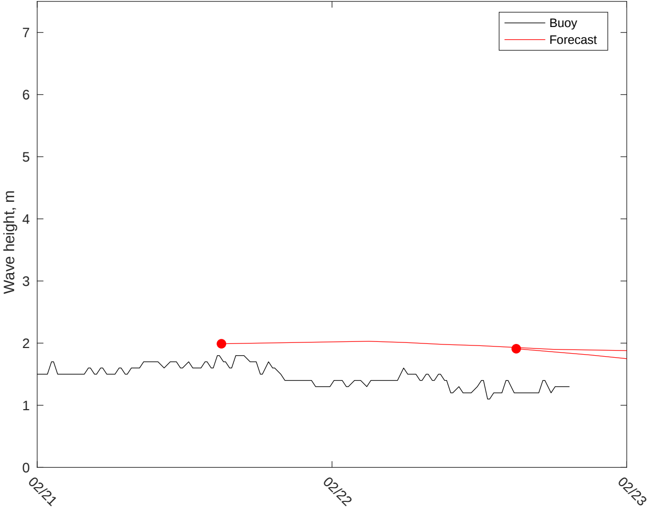
NDBC 46053 vs GFS Waves: 10 to 16 day forecast
