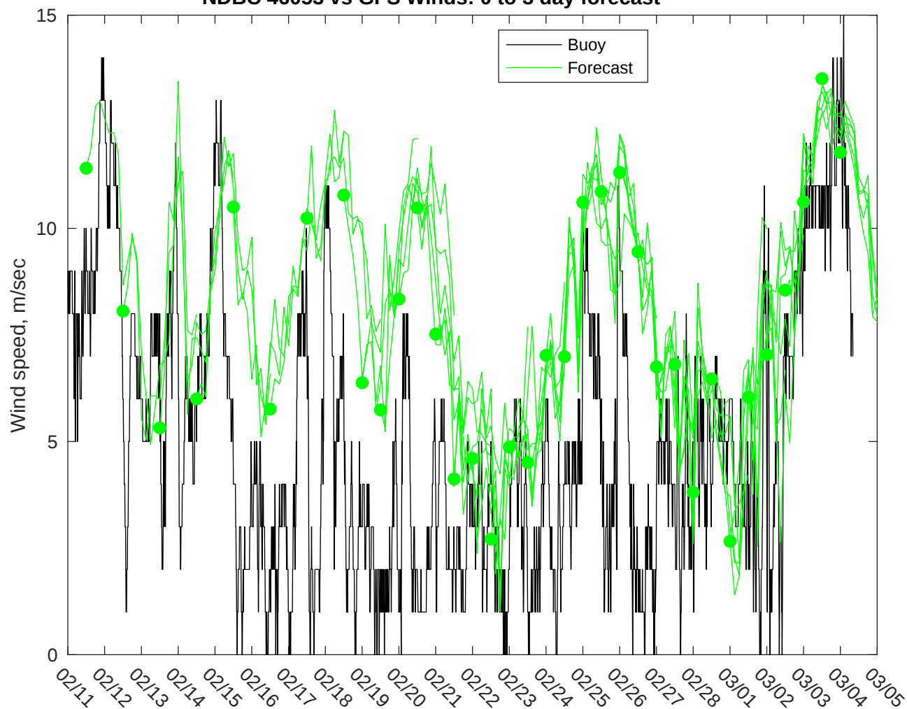
NDBC 46053 vs GFS Winds: 0 to 3 day forecast
