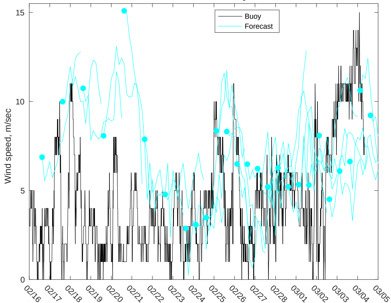
NDBC 46053 vs GFS Winds: 5 to 7 day forecast
