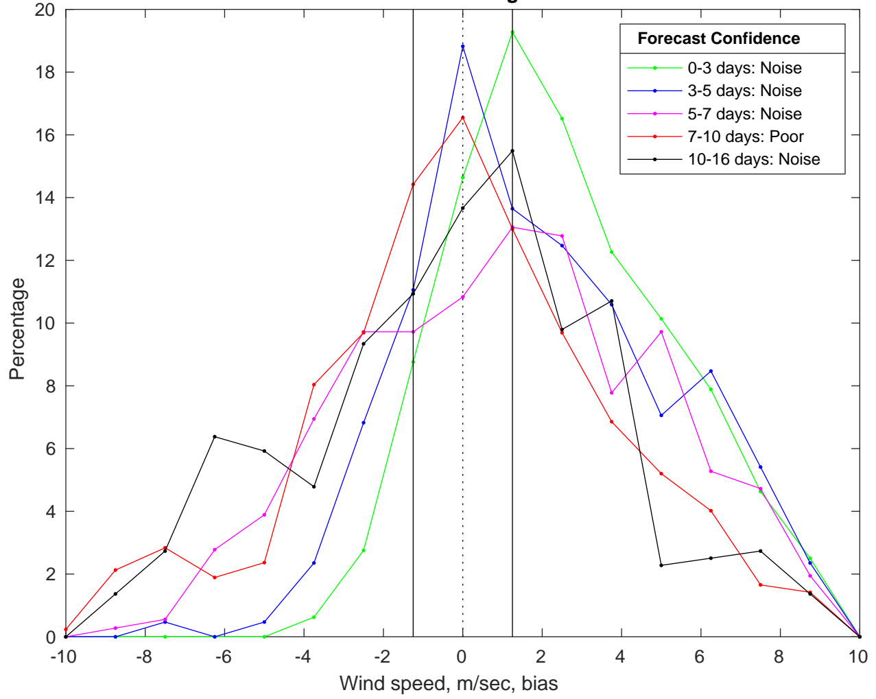
NDBC 46053 vs GFS Winds Bias Histogram: 04-Mar-2025
