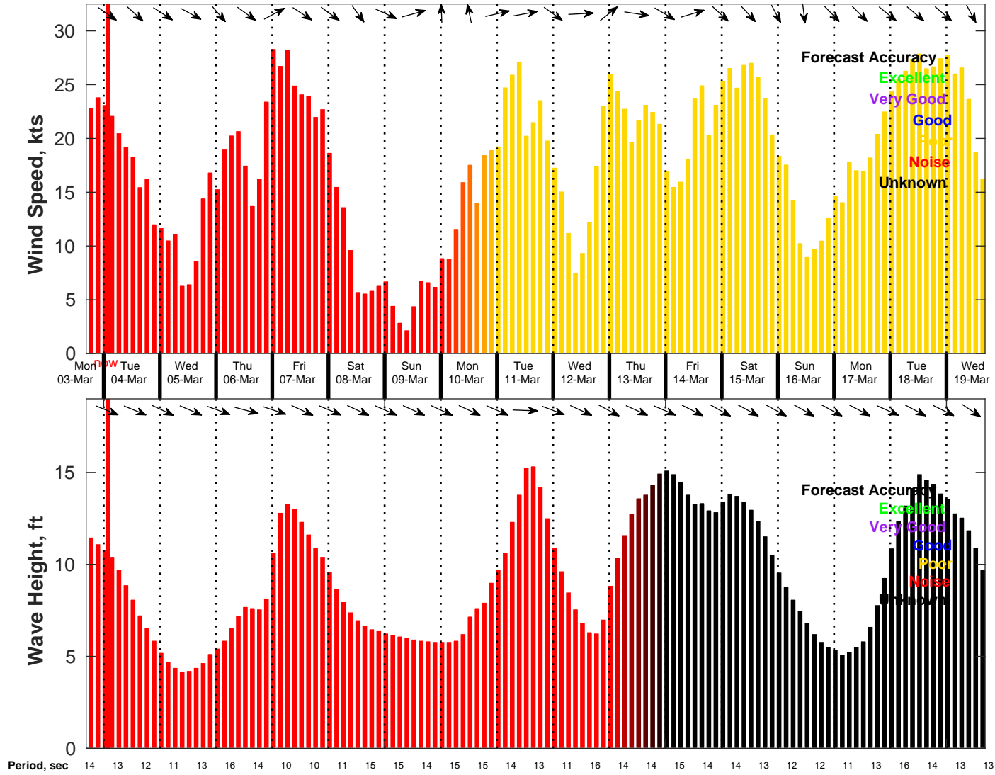
Wind & Wave Forecast for NDBC 46053 from 03-Mar-2025 17:00:00 to 19-Mar-2025 17:00:00
