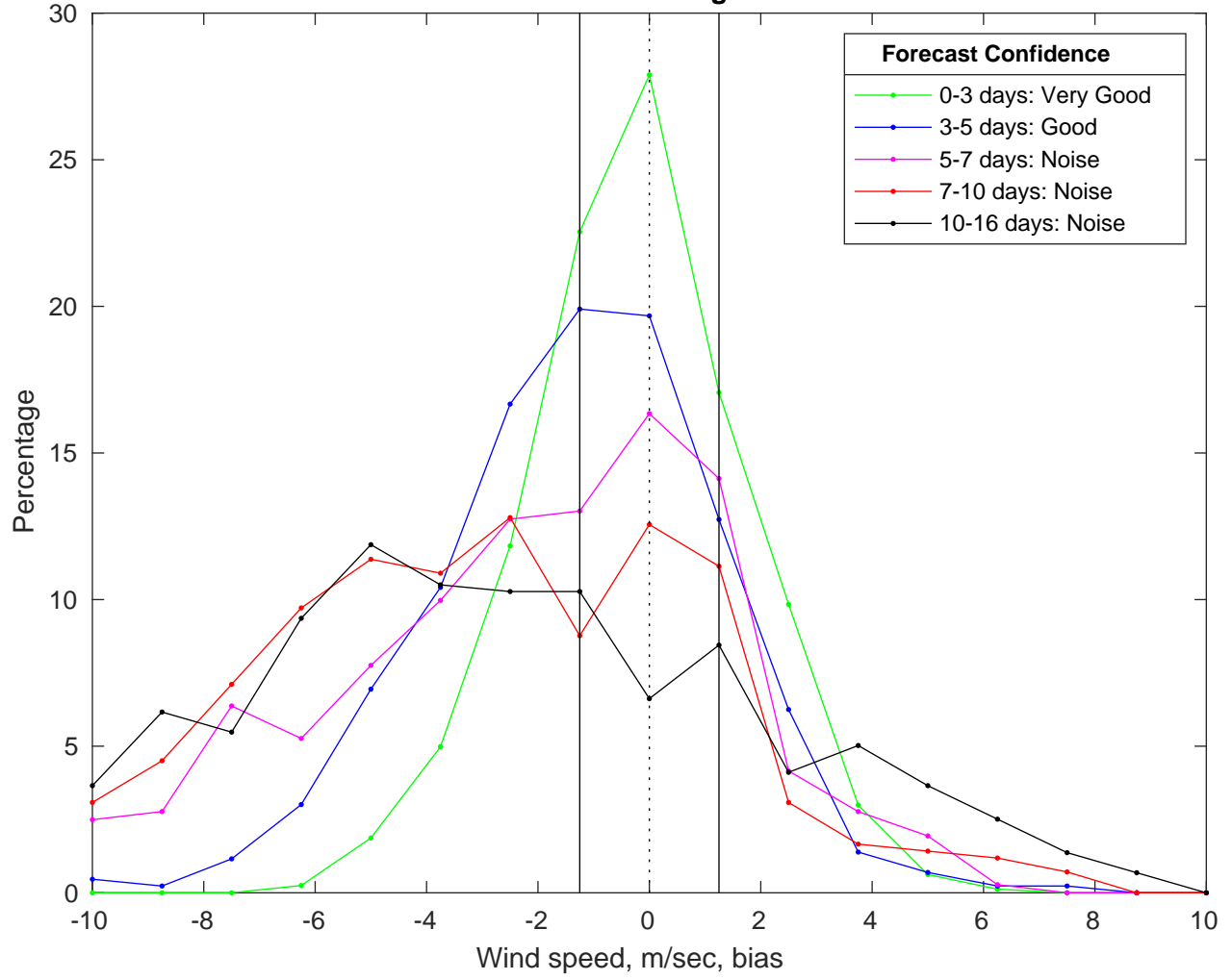
NDBC 46054 vs GFS Winds Bias Histogram: 04-Mar-2025
