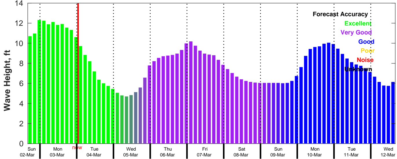
CMEMS Wave Forecast for NDBC 46054 from 02-Mar-2025 16:00:00 to 12-Mar-2025 16:00:00
