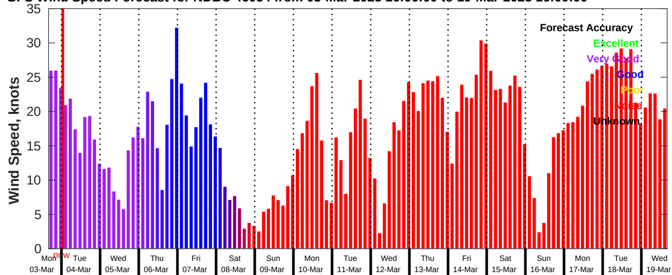
GFS Wind Speed Forecast for NDBC 46054 from 03-Mar-2025 16:00:00 to 19-Mar-2025 16:00:00
