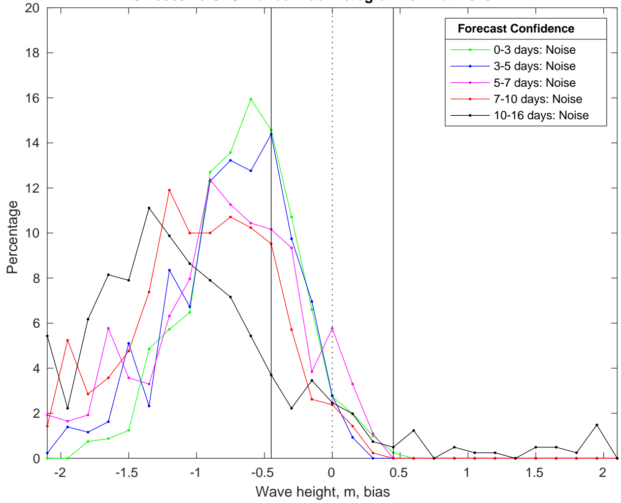
NDBC 46069 vs GFS Waves Bias Histogram: 04-Mar-2025
