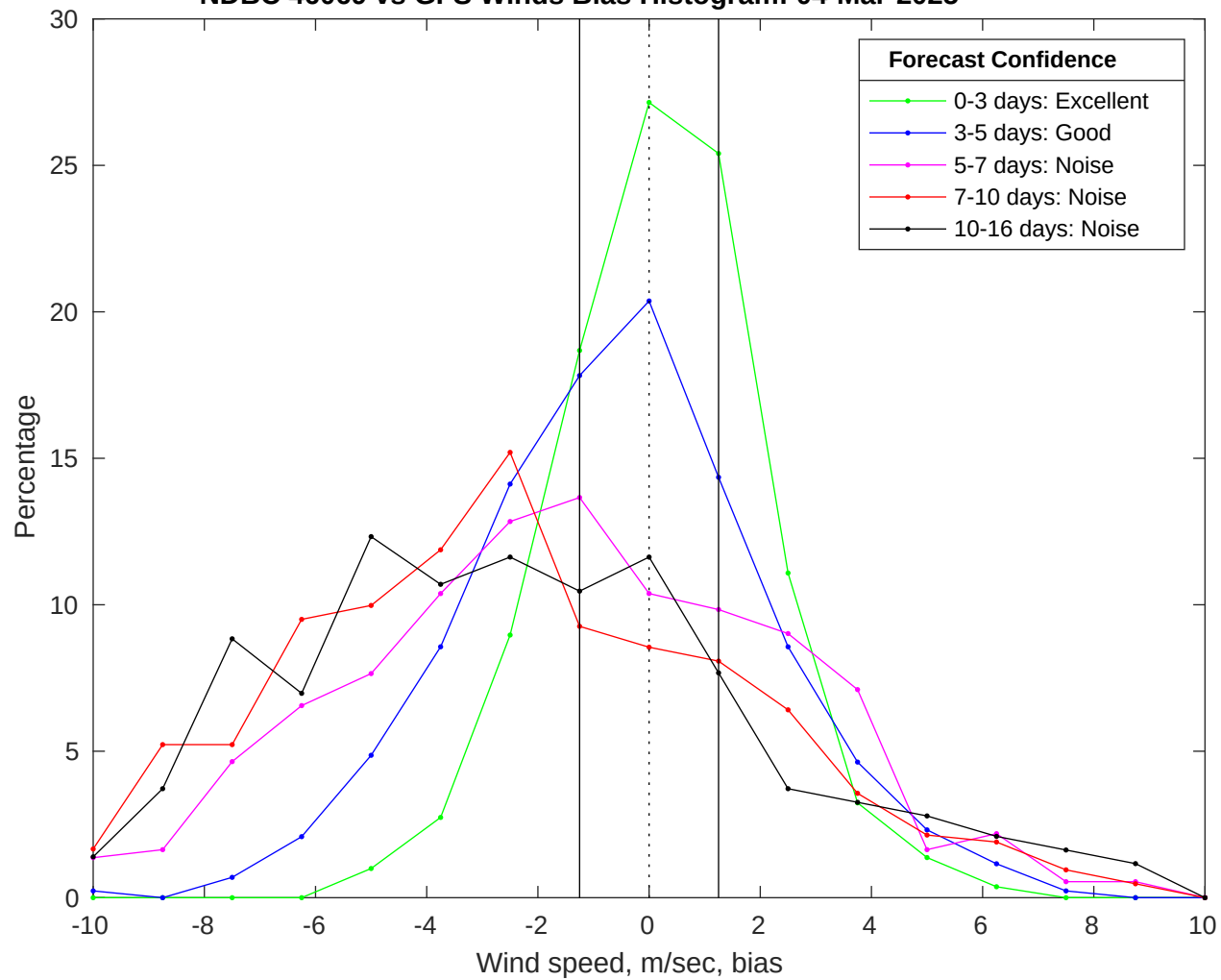
NDBC 46069 vs GFS Winds Bias Histogram: 04-Mar-2025
