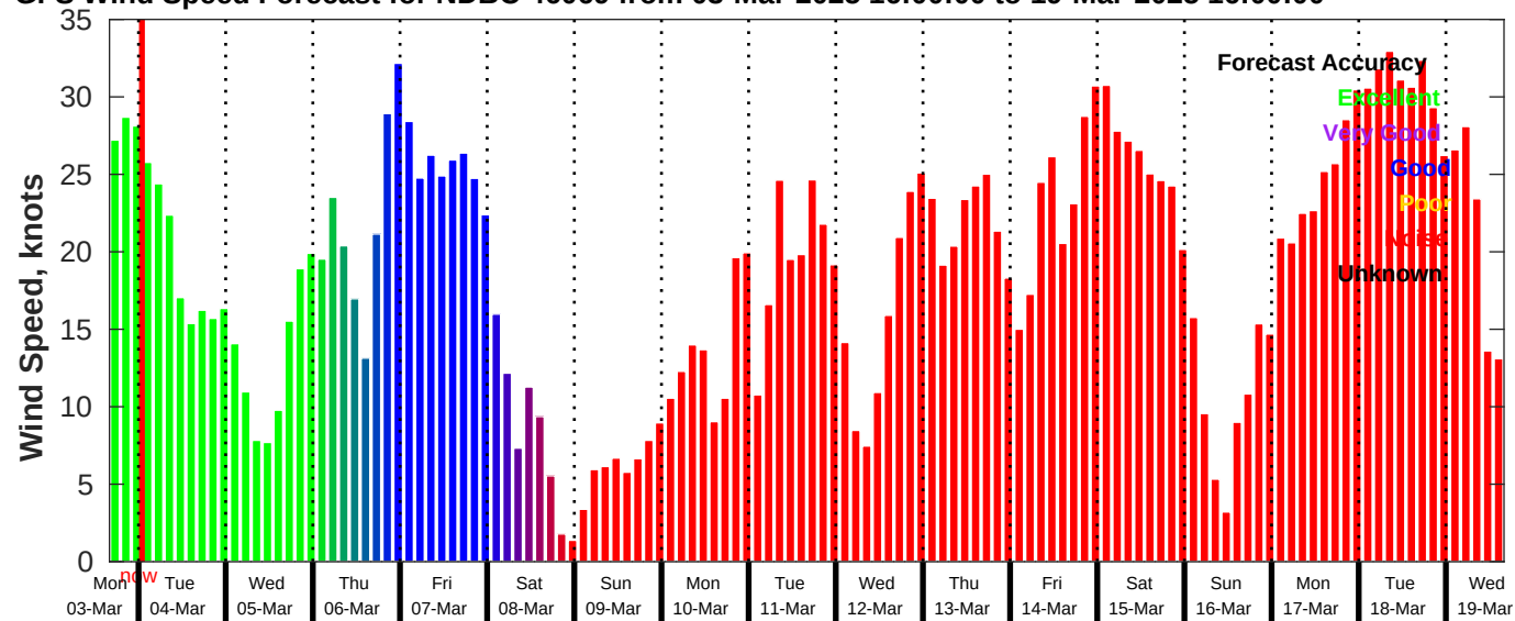
GFS Wind Speed Forecast for NDBC 46069 from 03-Mar-2025 16:00:00 to 19-Mar-2025 16:00:00
