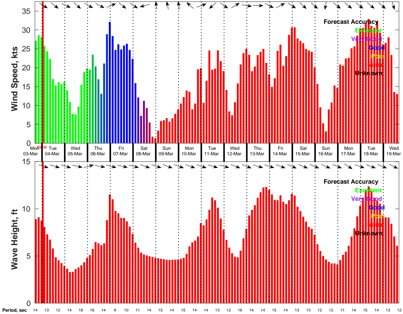
Wind & Wave Forecast for NDBC 46069 from 03-Mar-2025 16:00:00 to 19-Mar-2025 16:00:00
