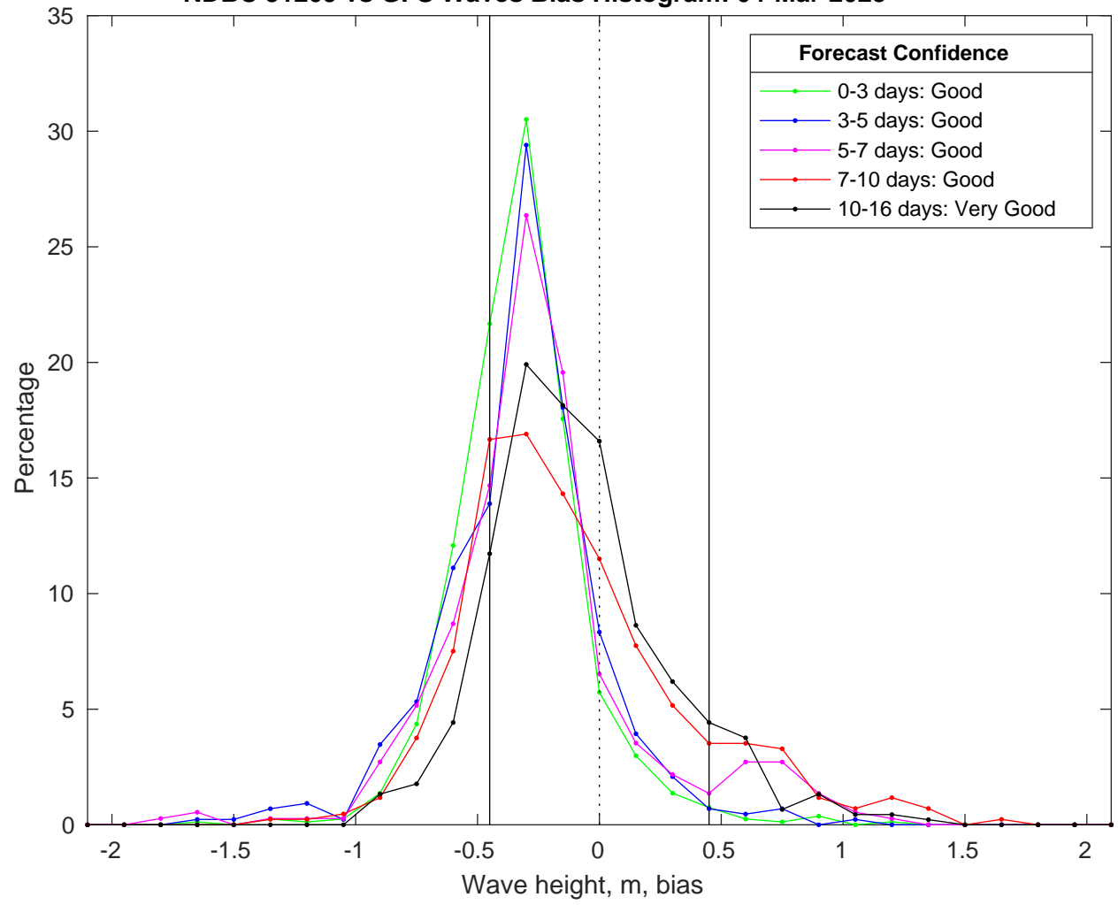
NDBC 51209 vs GFS Waves Bias Histogram: 04-Mar-2025
