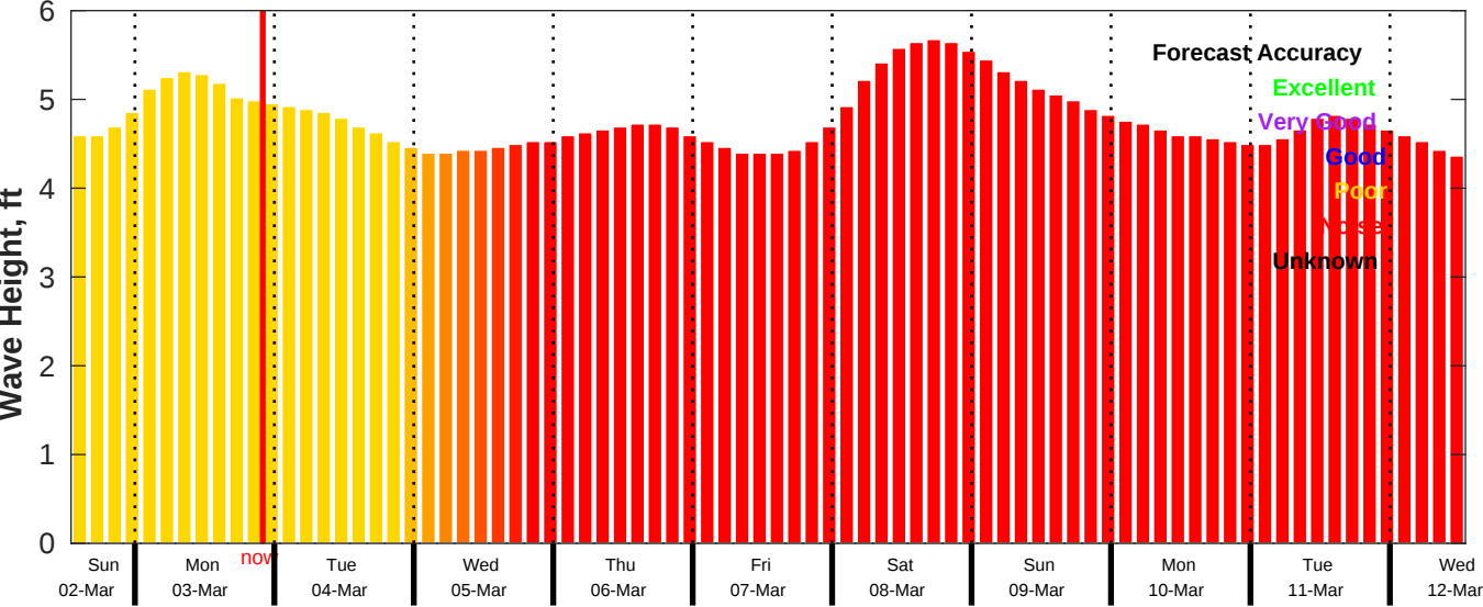
CMEMS Wave Forecast for NDBC 51209 from 02-Mar-2025 13:00:00 to 12-Mar-2025 13:00:00
