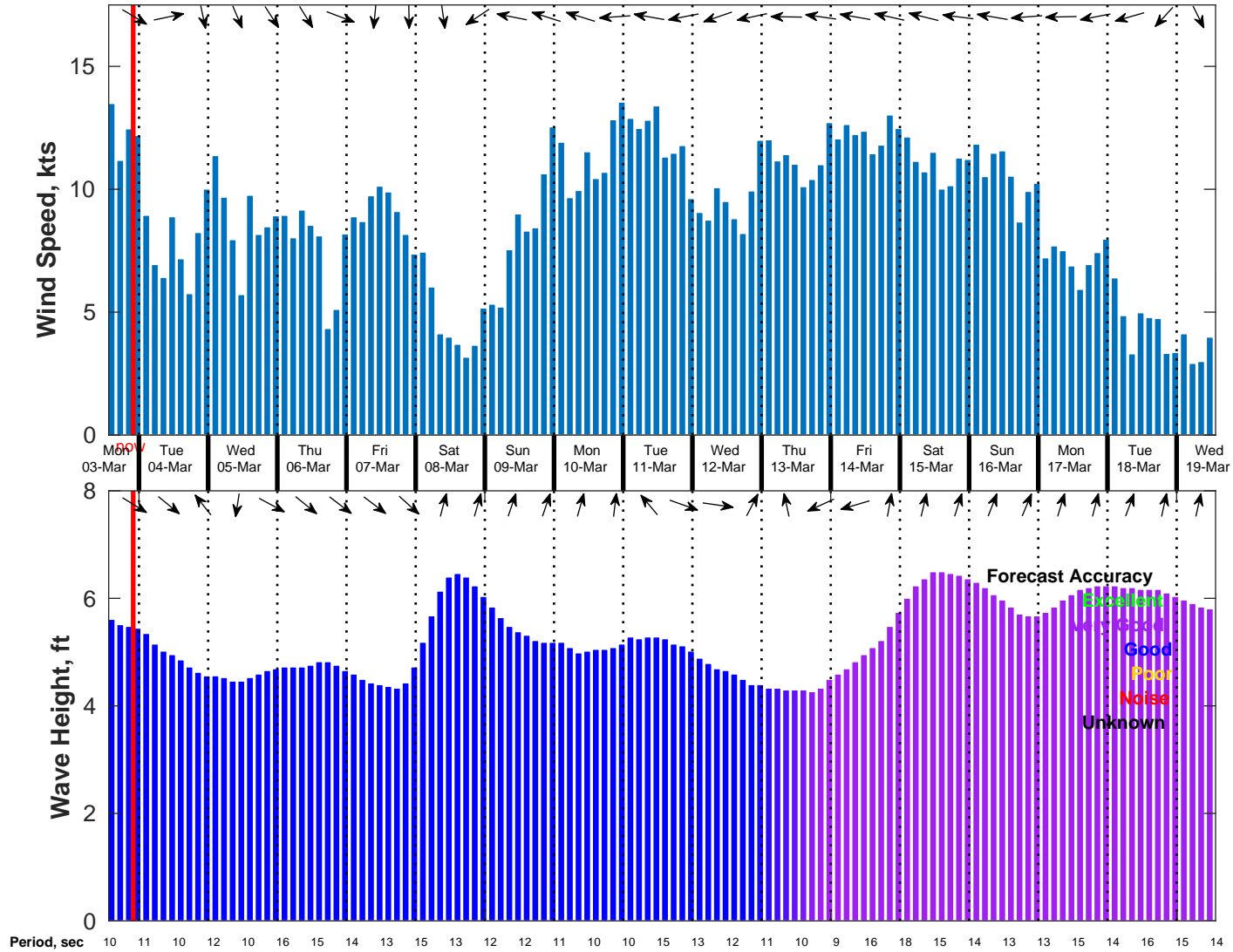
Wind & Wave Forecast for NDBC 51209 from 03-Mar-2025 13:00:00 to 19-Mar-2025 13:00:00
