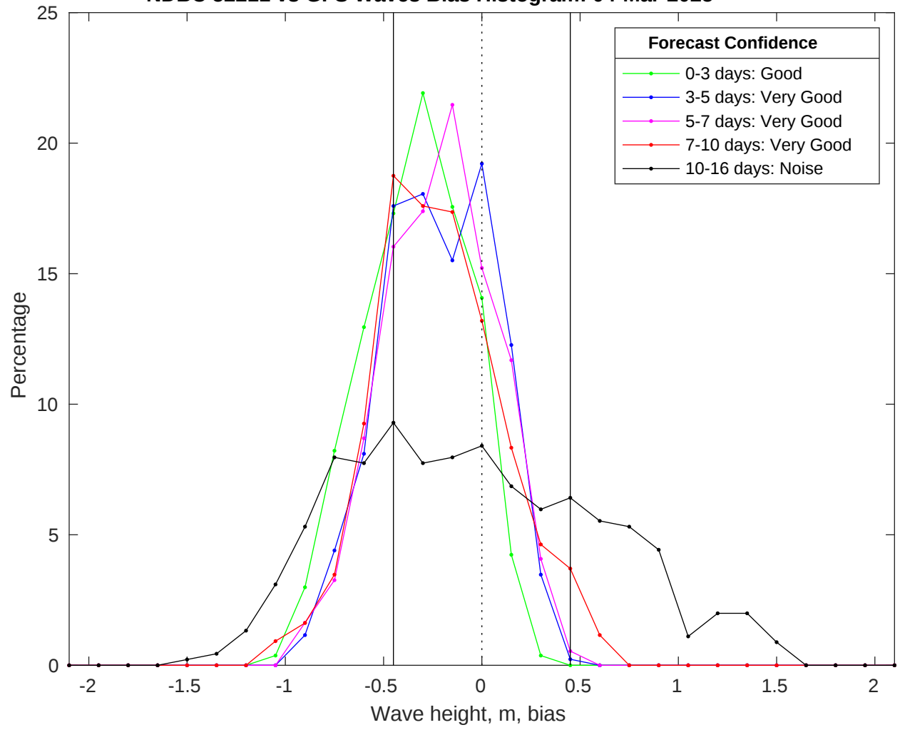
NDBC 52211 vs GFS Waves Bias Histogram: 04-Mar-2025
