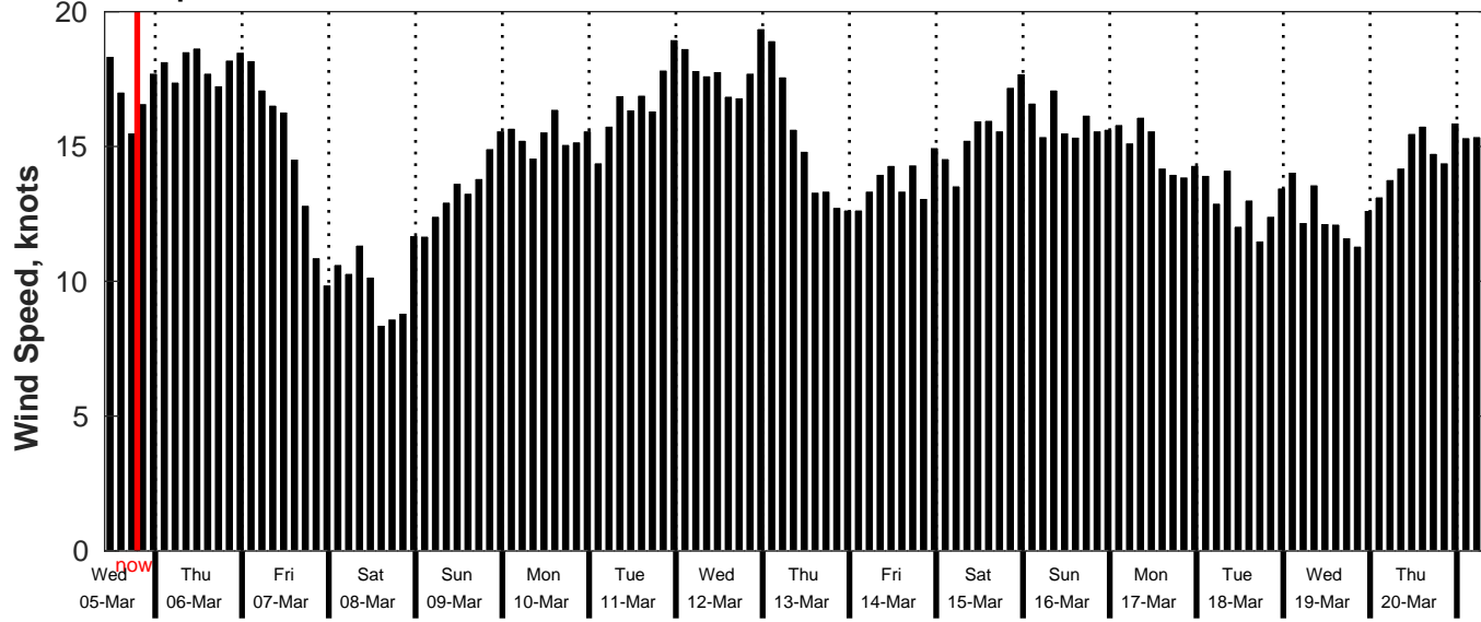
GFS Wind Speed Forecast for NDBC 52211 from 04-Mar-2025 10:00:00 to 20-Mar-2025 10:00:00
