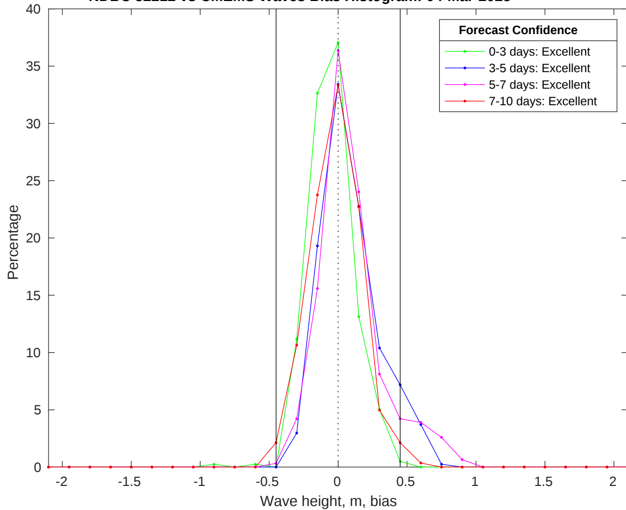
NDBC 52212 vs CMEMS Waves Bias Histogram: 04-Mar-2025
