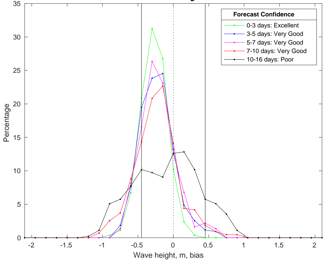
NDBC 52212 vs GFS Waves Bias Histogram: 04-Mar-2025
