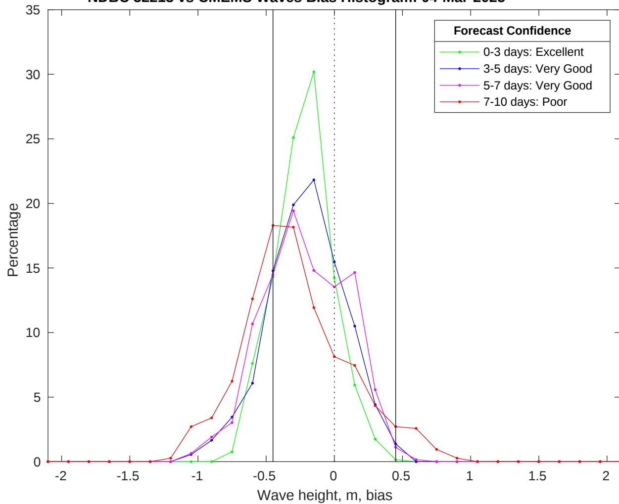
NDBC 52213 vs CMEMS Waves Bias Histogram: 04-Mar-2025
