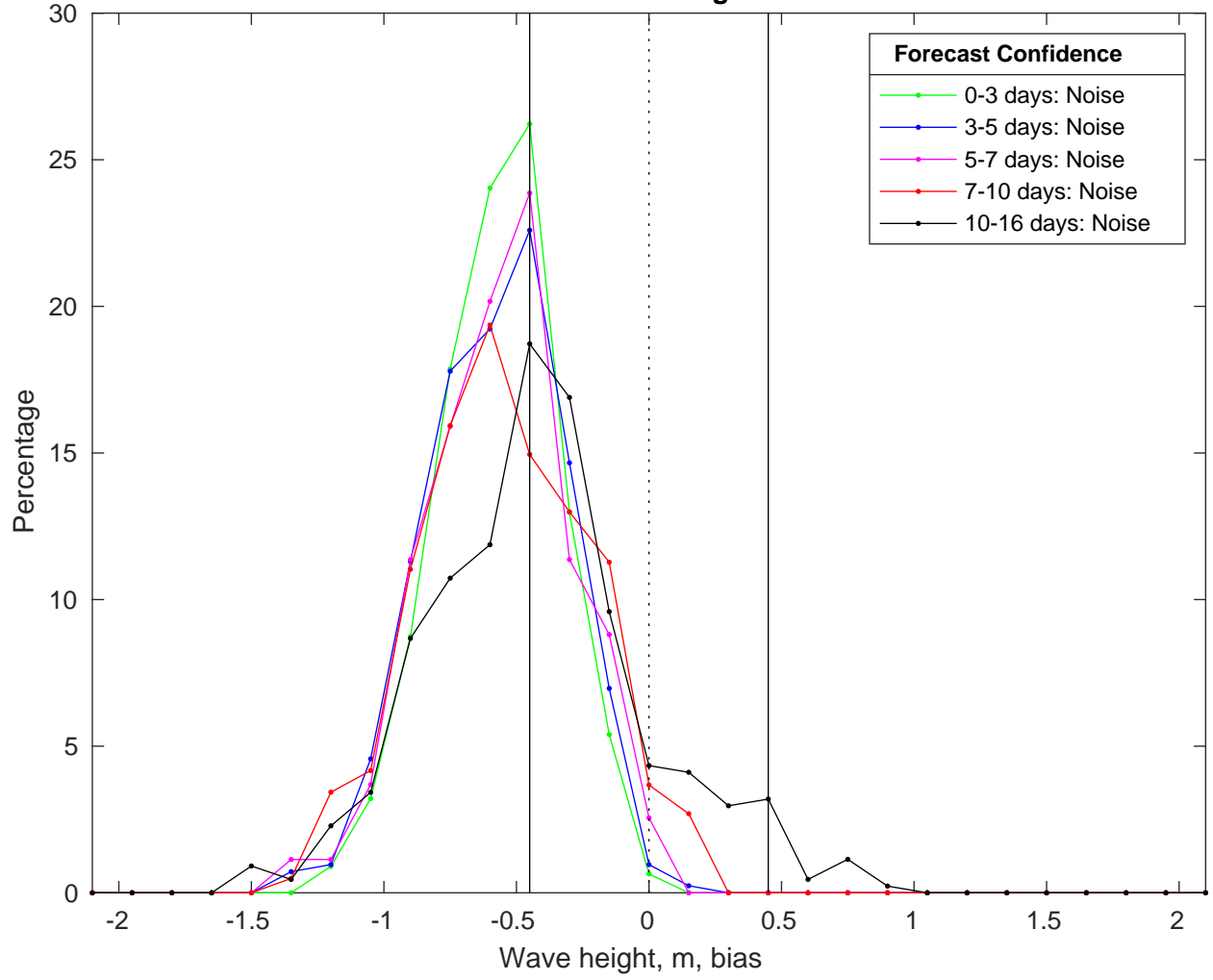
NDBC 52213 vs GFS Waves Bias Histogram: 04-Mar-2025
