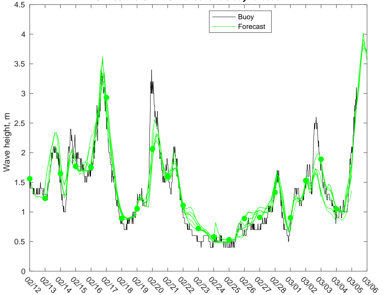
NDBC 41004 vs CMEMS Waves: 0 to 3 day forecast
