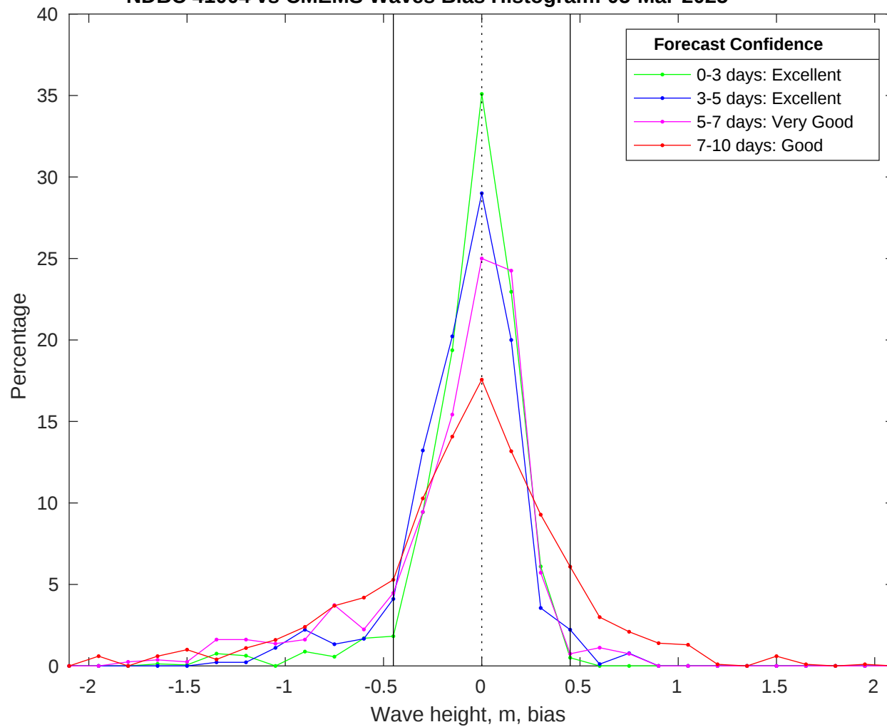
NDBC 41004 vs CMEMS Waves Bias Histogram: 05-Mar-2025
