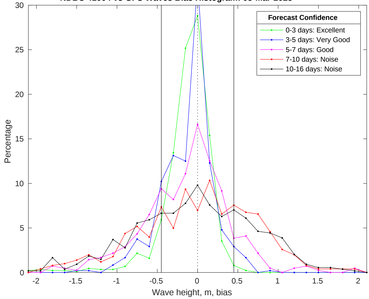
NDBC 41004 vs GFS Waves Bias Histogram: 05-Mar-2025
