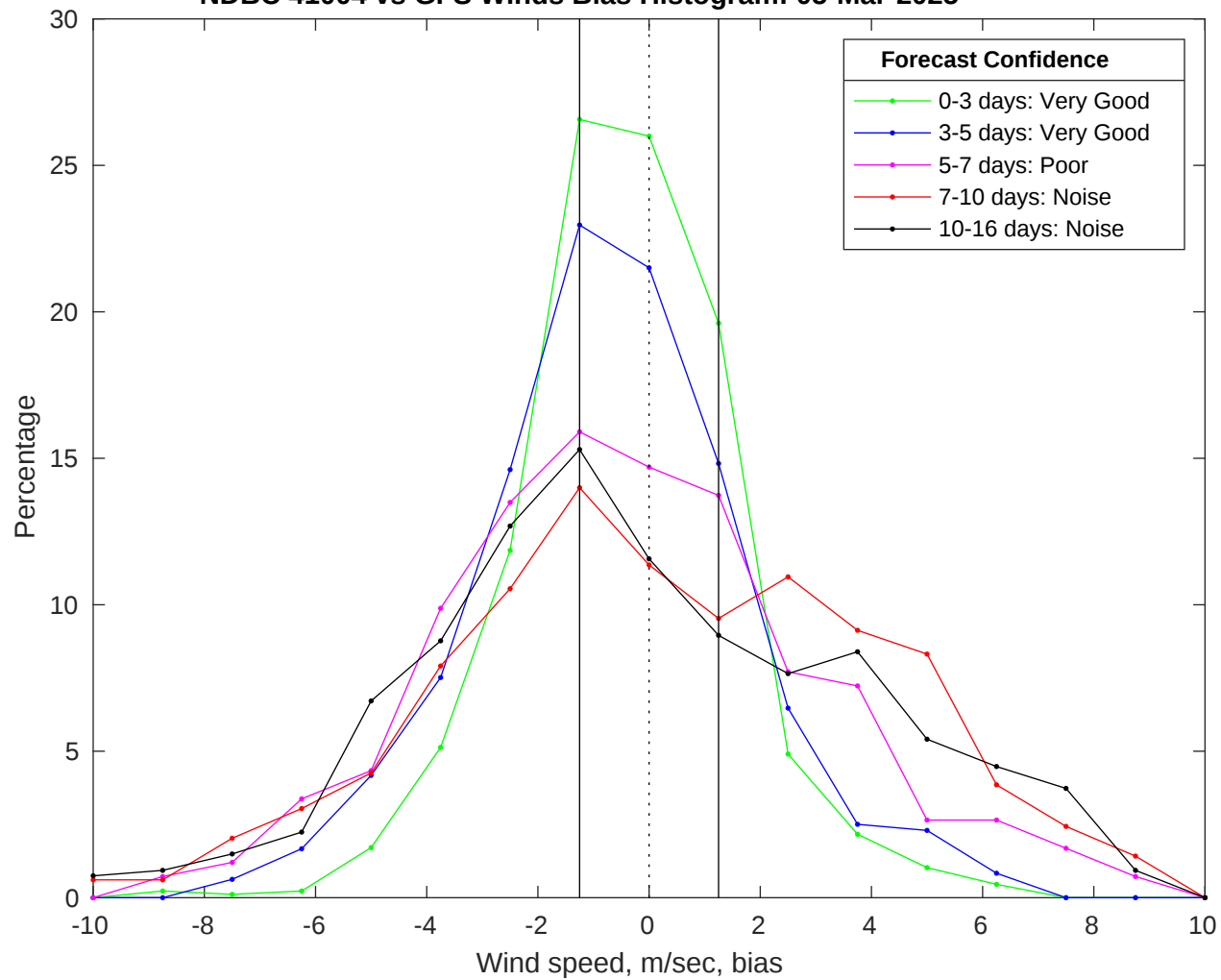
NDBC 41004 vs GFS Winds Bias Histogram: 05-Mar-2025
