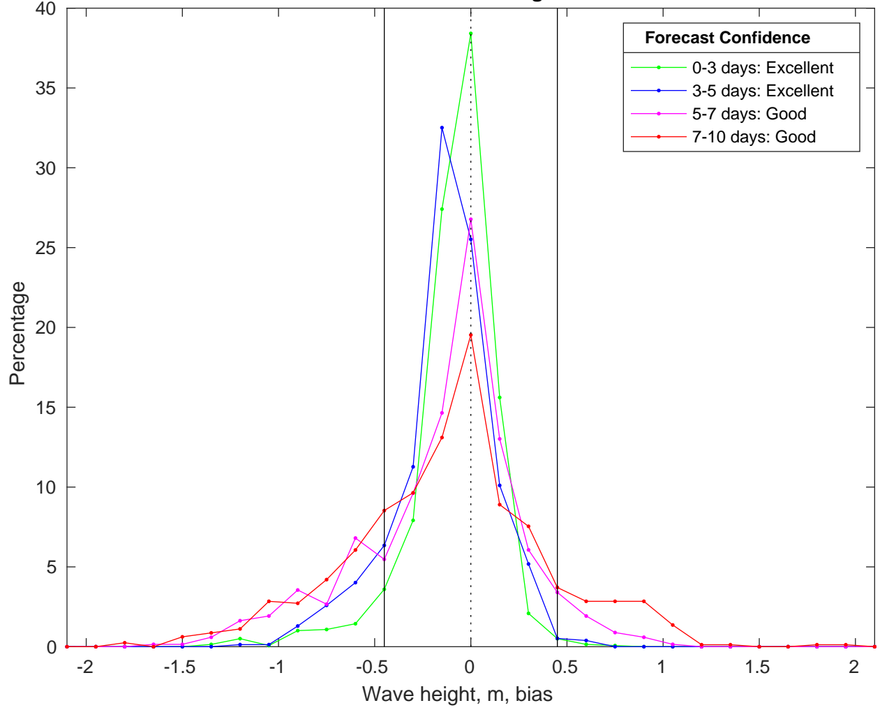
NDBC 41013 vs CMEMS Waves Bias Histogram: 05-Mar-2025
