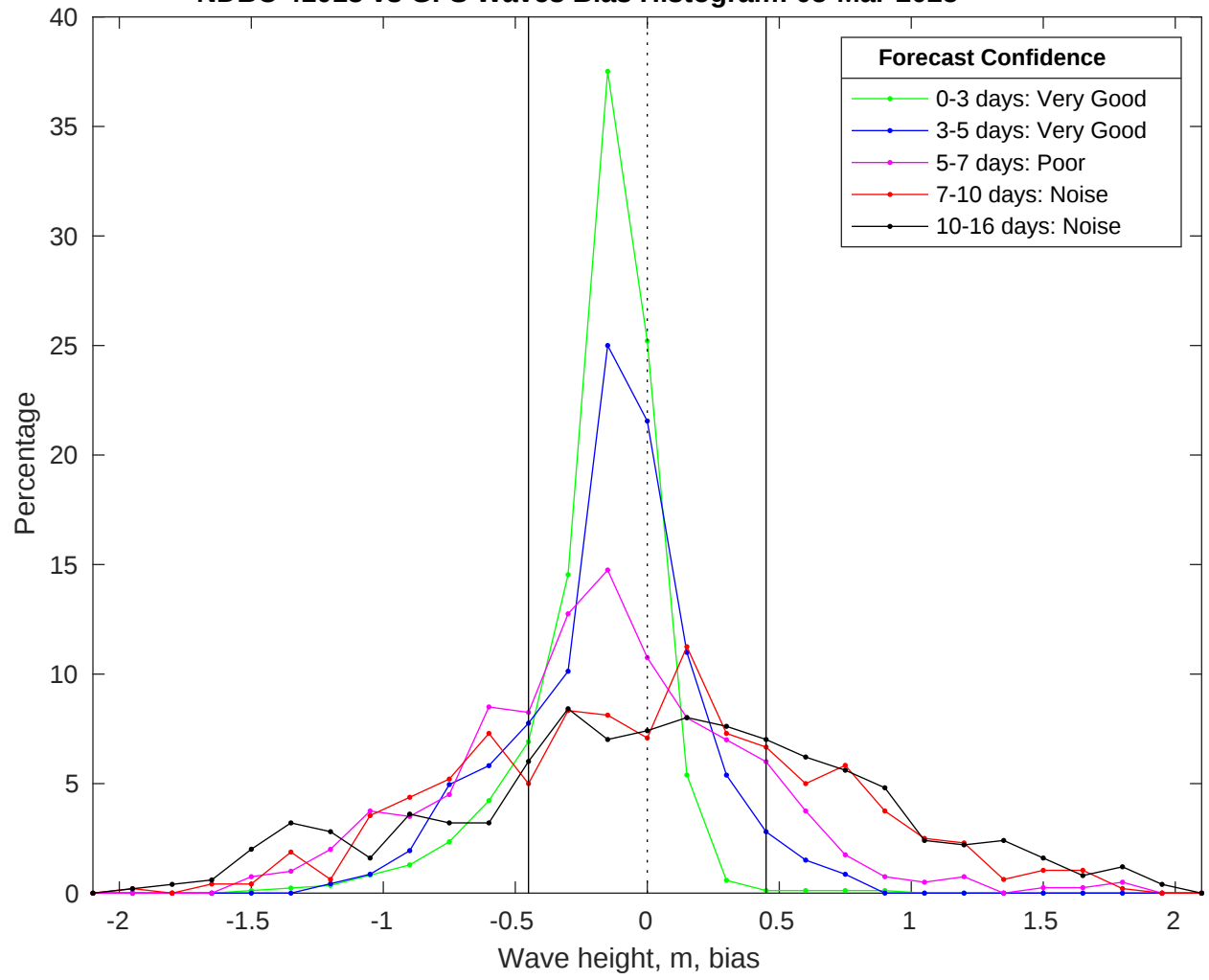
NDBC 41013 vs GFS Waves Bias Histogram: 05-Mar-2025
