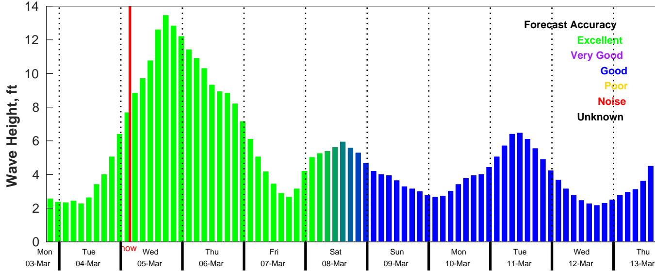
CMEMS Wave Forecast for NDBC 41013 from 03-Mar-2025 19:00:00 to 13-Mar-2025 19:00:00
