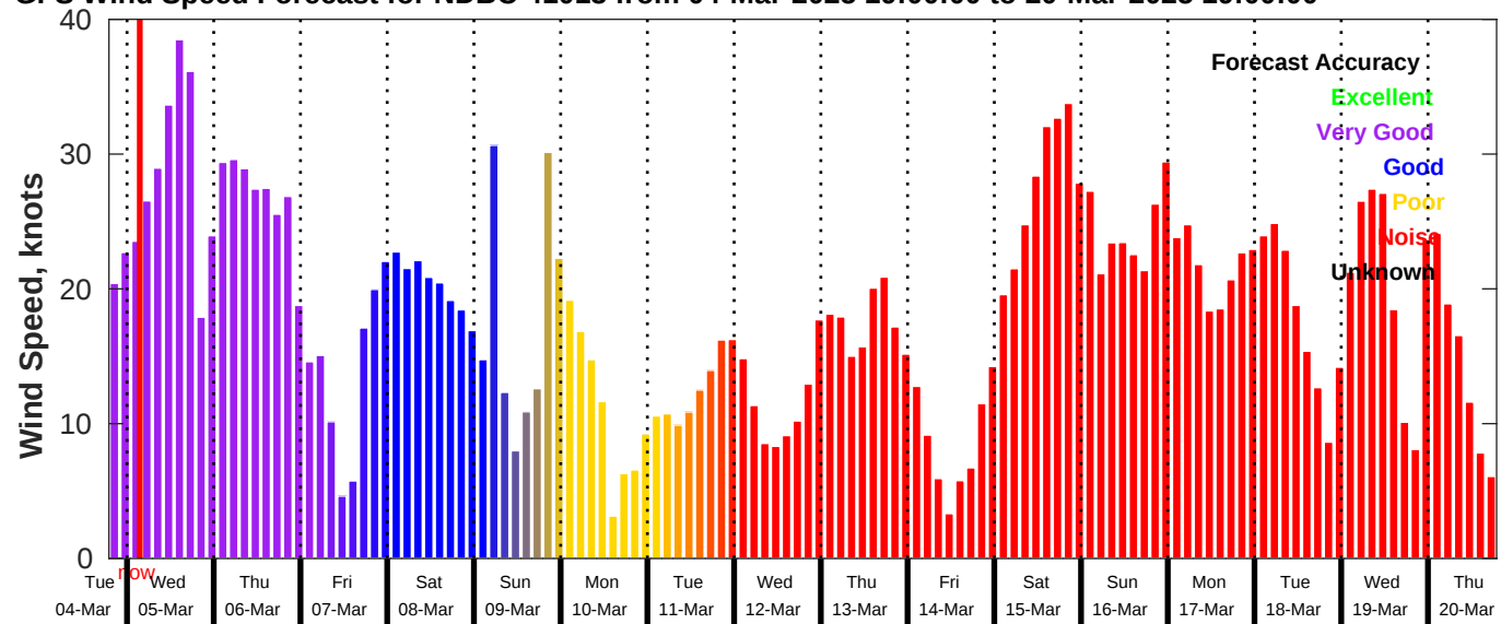
GFS Wind Speed Forecast for NDBC 41013 from 04-Mar-2025 19:00:00 to 20-Mar-2025 19:00:00
