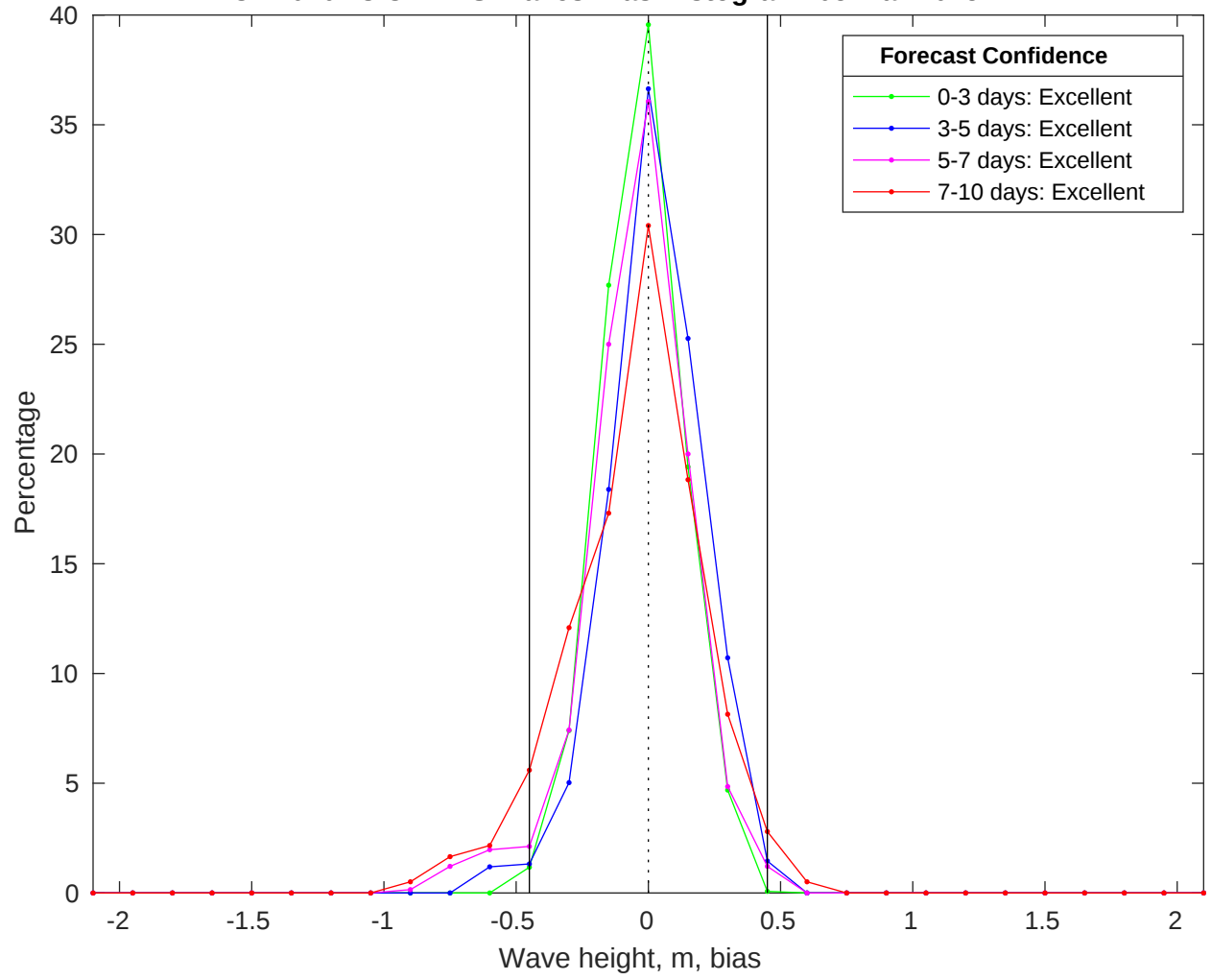
NDBC 41040 vs CMEMS Waves Bias Histogram: 05-Mar-2025
