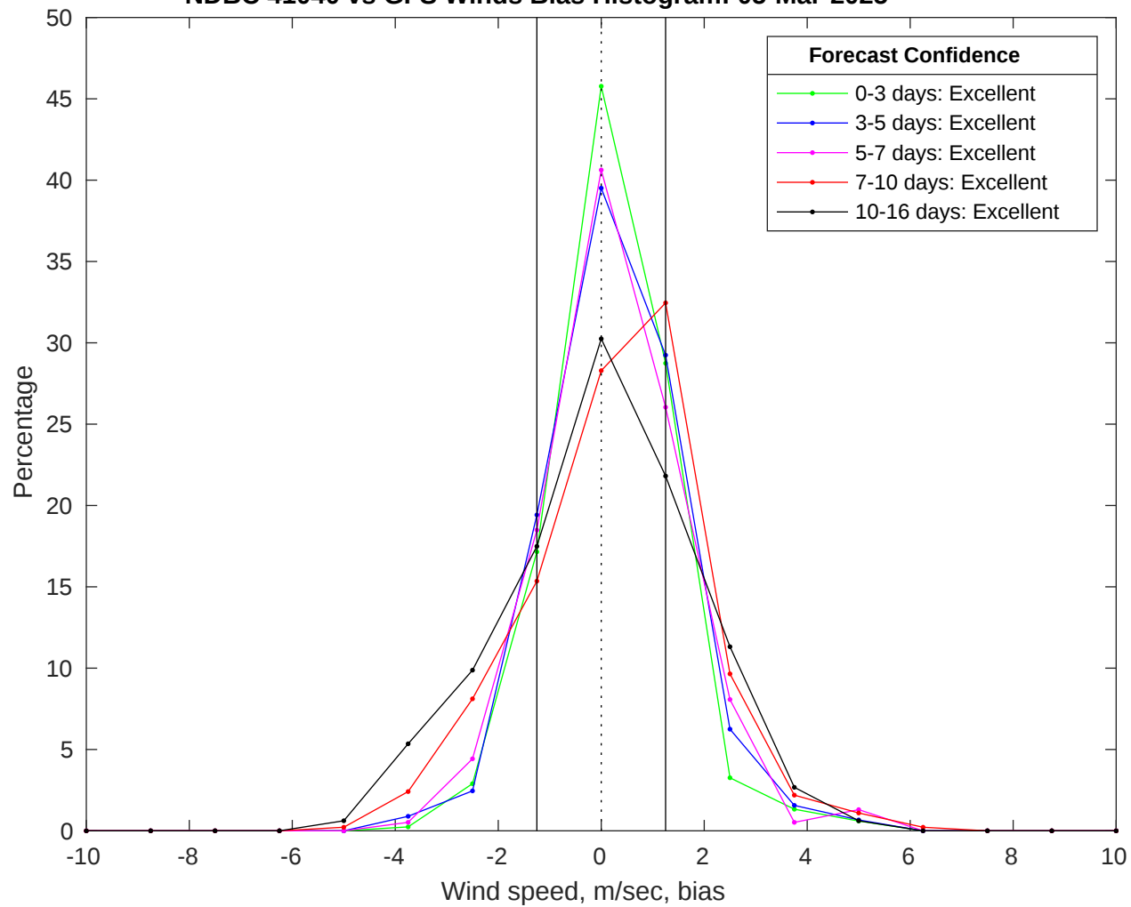
NDBC 41040 vs GFS Winds Bias Histogram: 05-Mar-2025
