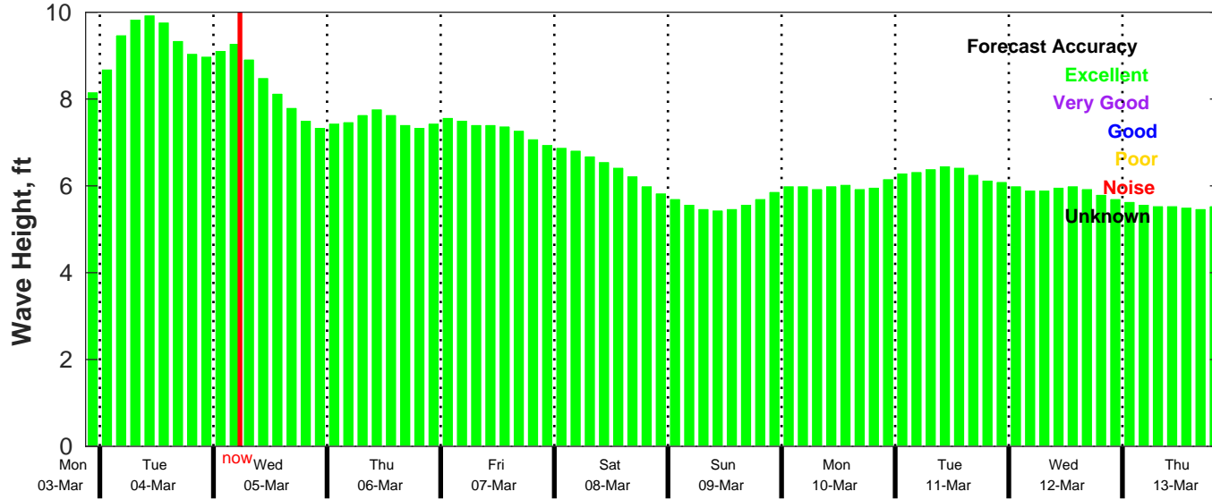
CMEMS Wave Forecast for NDBC 41040 from 03-Mar-2025 21:00:00 to 13-Mar-2025 21:00:00
