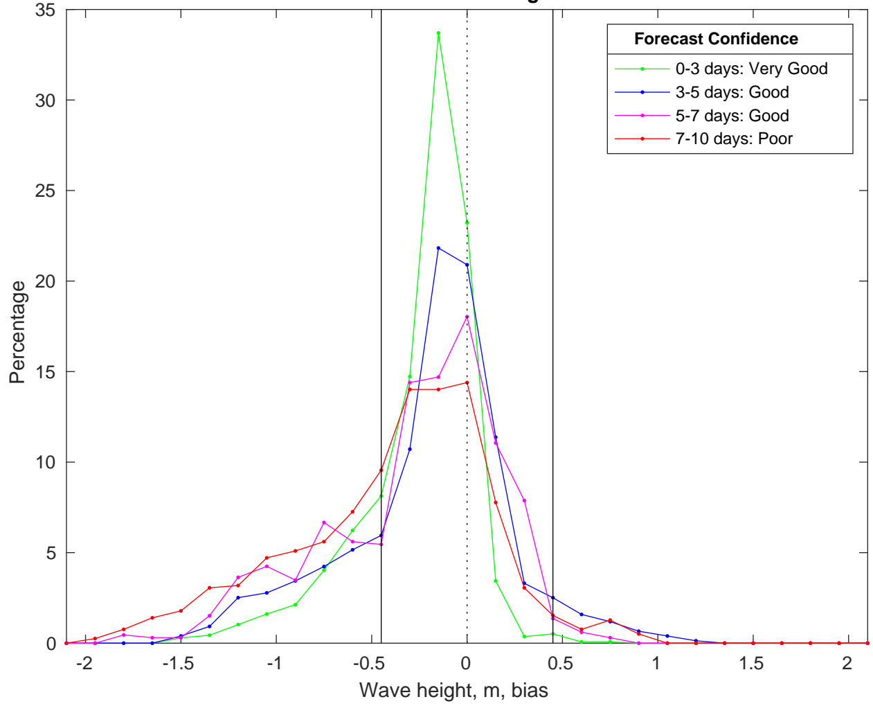
NDBC 42019 vs CMEMS Waves Bias Histogram: 05-Mar-2025
