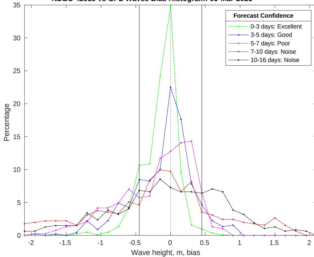
NDBC 42019 vs GFS Waves Bias Histogram: 05-Mar-2025
