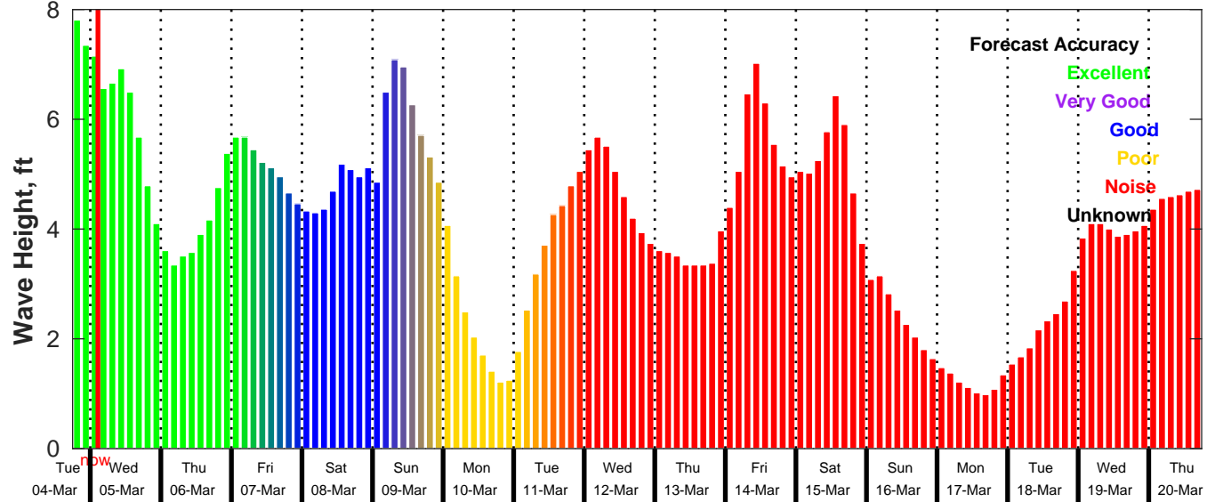
GFS Wave Forecast for NDBC 42019 from 04-Mar-2025 18:00:00 to 20-Mar-2025 18:00:00
