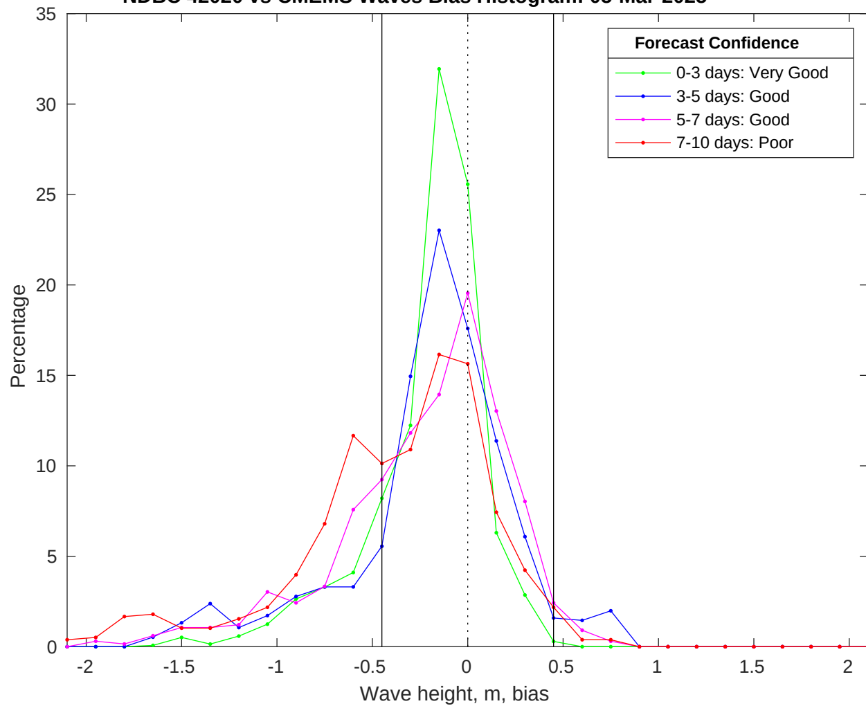
NDBC 42020 vs CMEMS Waves Bias Histogram: 05-Mar-2025
