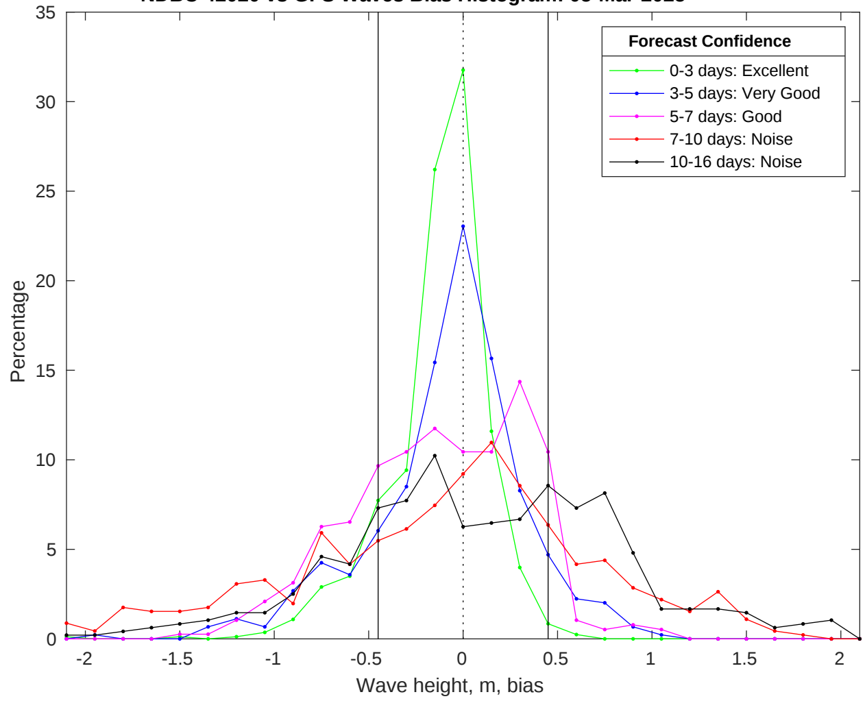
NDBC 42020 vs GFS Waves Bias Histogram: 05-Mar-2025
