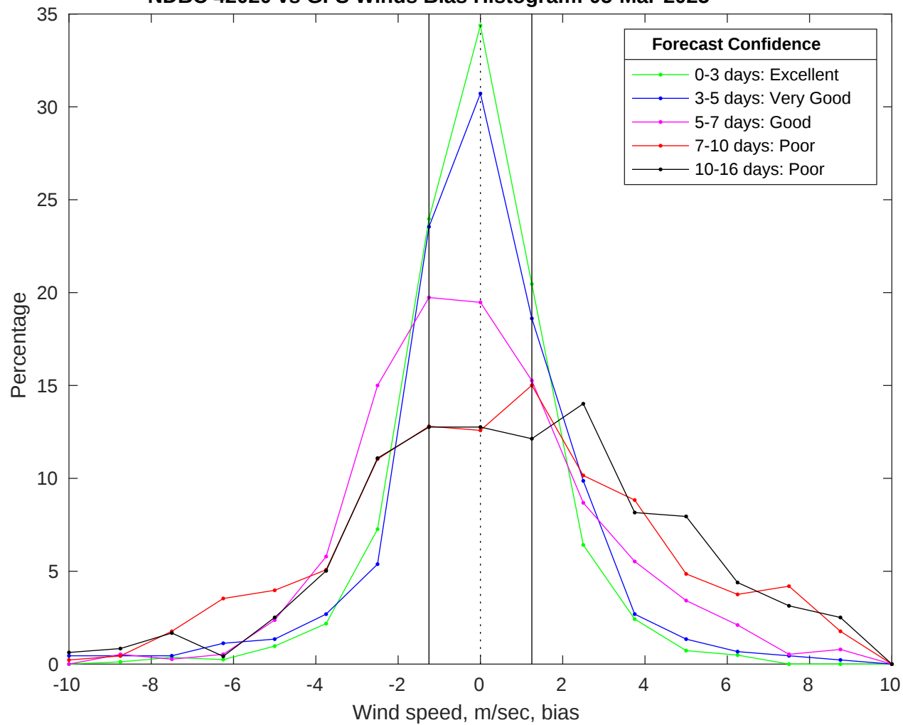
NDBC 42020 vs GFS Winds Bias Histogram: 05-Mar-2025
